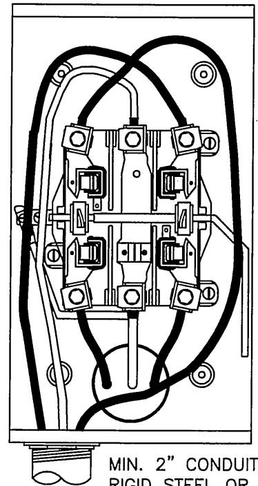
WIRING DIAGRAM FOR UNDERGROUND
