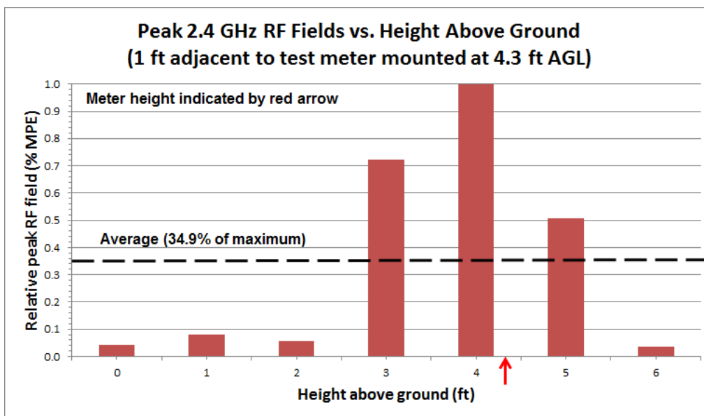
Figure 27. Relative peak 2.4 GHz band RF field (as a percent of the MPE) vs. height above ground at one foot in front of the Elster test meters. Measured field was normalized to the greatest value determined from all measurements.
