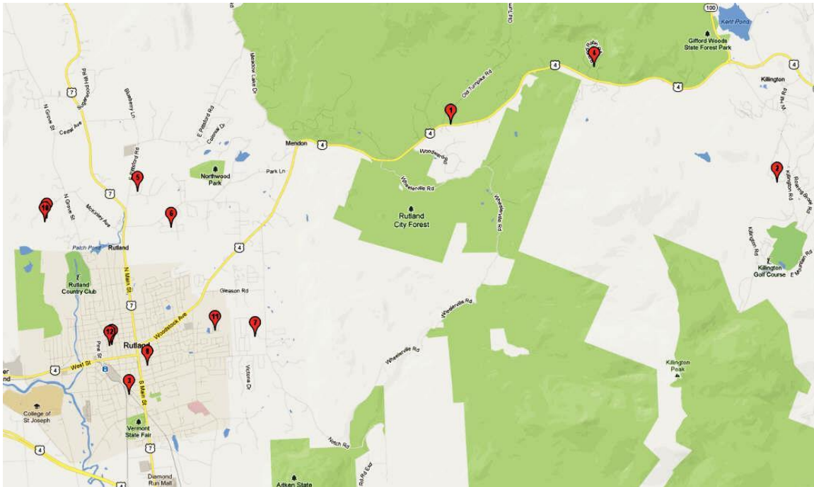
Figure 3. Smart meter measurement locations (13 total) in the Rutland, VT GMP service territory. Sites 9 and 10 and 12 and 13 are close together.
