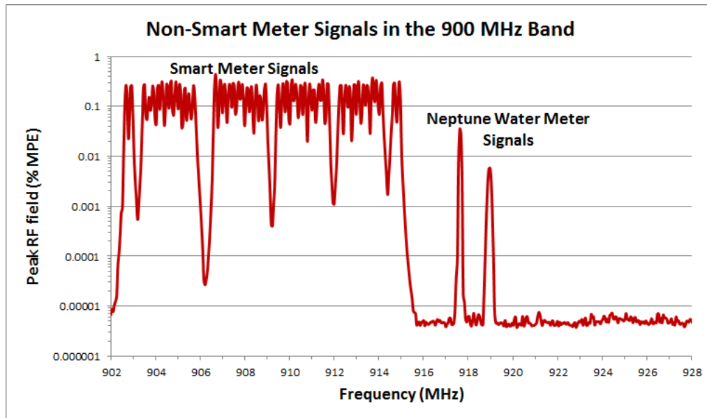
Figure 70. Spectrum measurement result at GMP site 4 where RF fields above the frequency range in which the Elster meter operates are apparent. The signals are intermittent and appear approximately once every 14 seconds.
