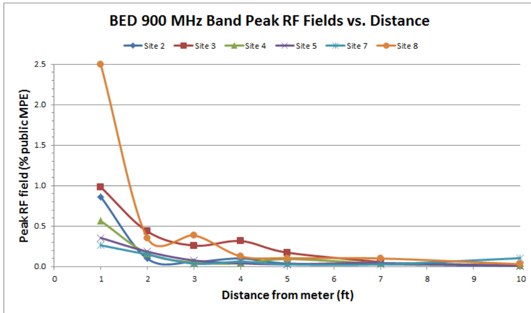
Figure 16. Linear display of measured peak values of RF fields at distances up to 10 feet in front of individual smart meters operated by BED.
