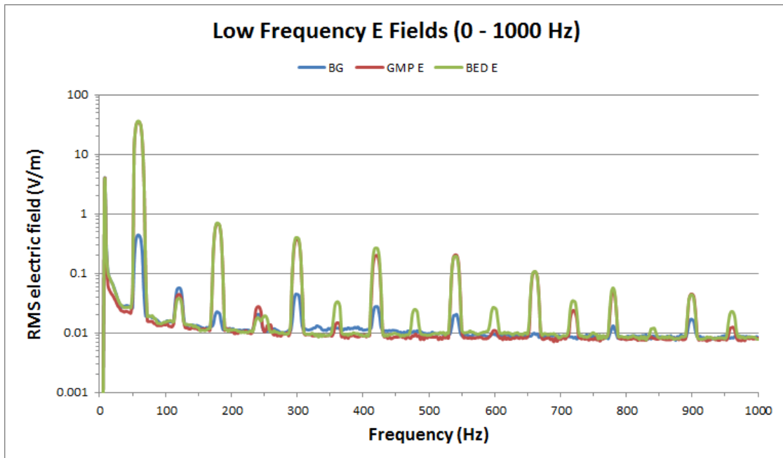
Figure 49. Low frequency electric (E) fields measured in the range of 0 to 1,000 Hz (1 kHz) for the GMP Elster meter, the BED Itron meter and background.
