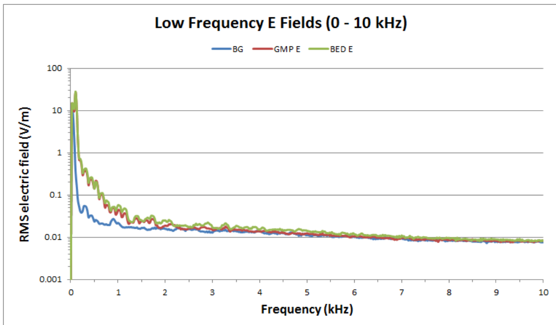
Figure 50. Low frequency electric (E) fields measured in the range of 0 to 10 kHz for the GMP Elster meter, the BED Itron meter and background.
