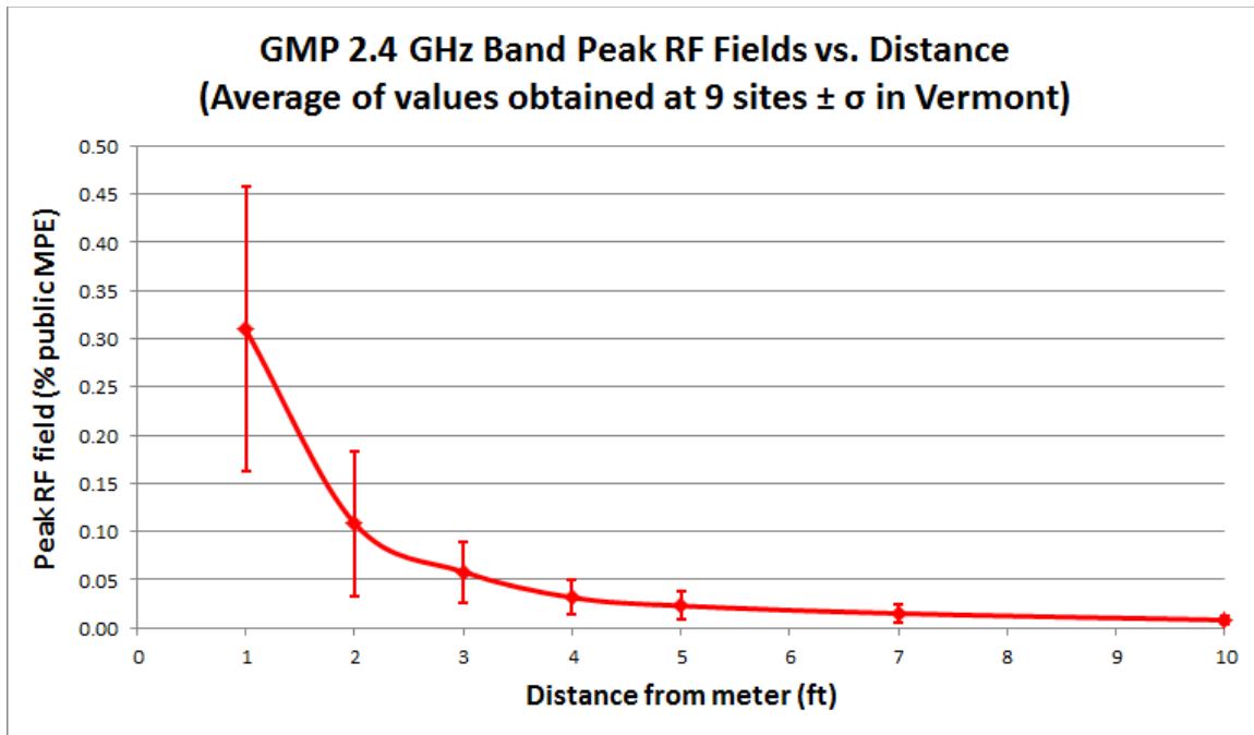
Figure 24. Average of 2.4 GHz band peak RF fields vs. distance \pm 1 standard deviation of values obtained at nine individual smart meter sites in the GMP service territory.
