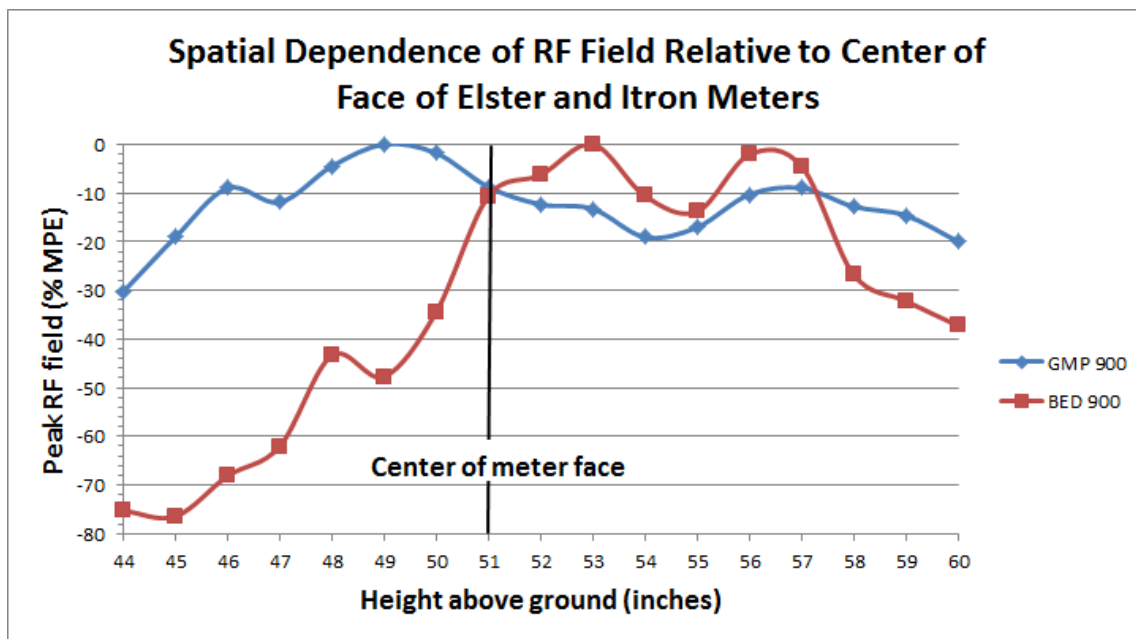
Figure 72. The measured spatial dependence of 900 MHz band RF fields produced at one foot from the GMP Elster and BED Itron smart meters along a vertical line extending from 44 inches to 60 inches above the floor.
