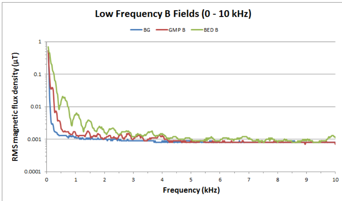
Figure 53. Low frequency magnetic flux density (B) measured in the range of 0 to 10 kHz for the GMP Elster meter, the BED Itron meter and background.
