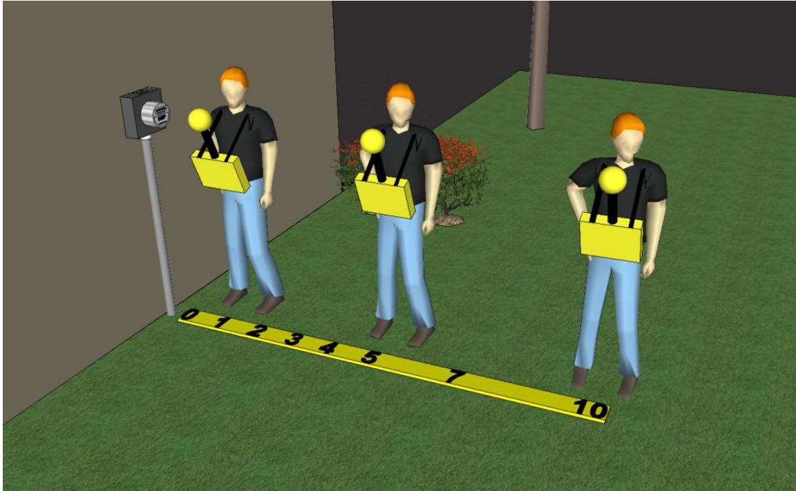
Figure 9. Illustration of the measurement of RF fields at different distances, ranging from one foot to 10 feet from the front surface of a smart meter.
