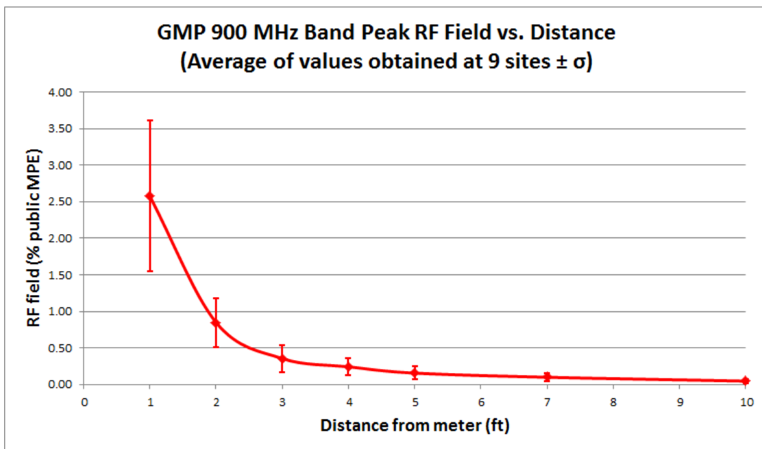
Figure 15. Average of 900 MHz band peak RF fields vs. distance \pm 1 standard deviation of values obtained at nine individual smart meter sites in the GMP Rutland area.
