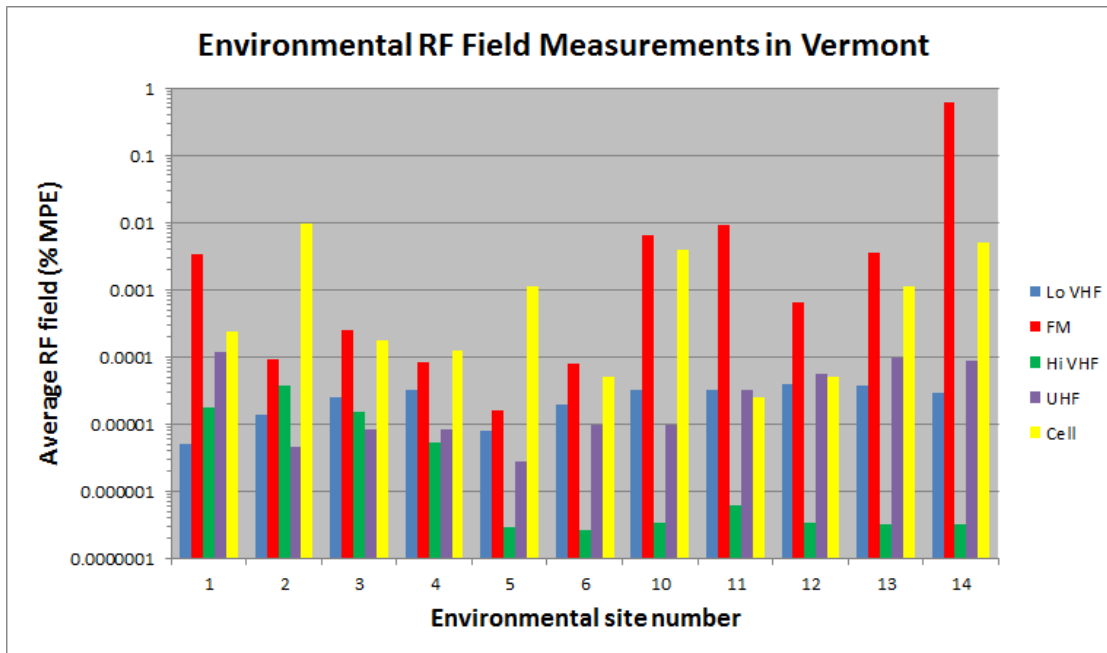
Figure 69. Graphical display of the integrated RF fields across five different frequency bands allocated to broadcast TV and FM radio as well as mobile phone base stations (wireless or cell band).
