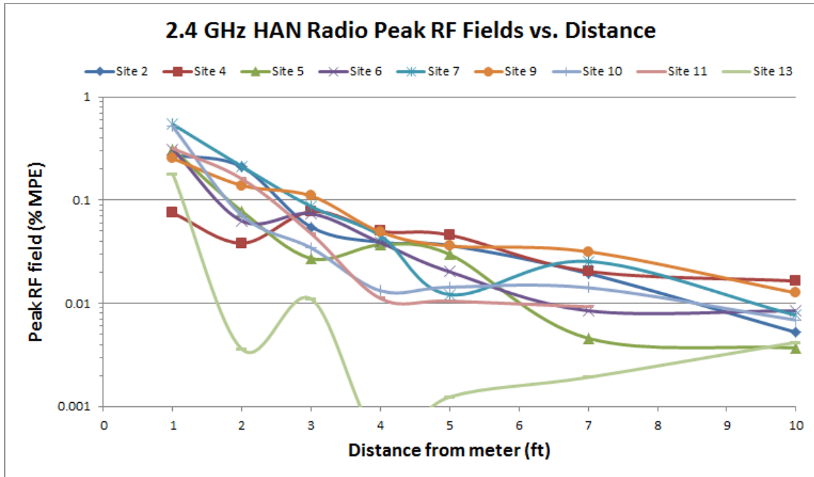
Figure 23. Logarithmic display of measured peak 2.4 GHz RF fields of the HAN radio at GMP smart meters observed at nine individual meter sites.
