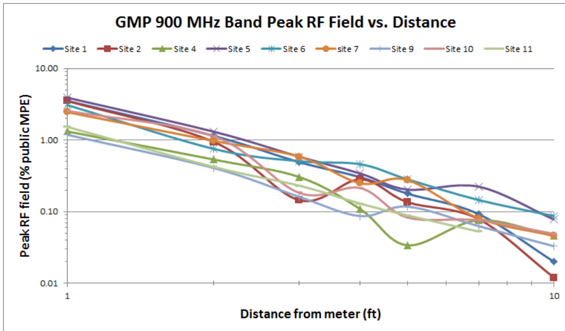
Figure 14. Logarithmic display of measured peak values of RF fields at distances up to 10 feet in front of individual smart meters operated by GMP.
