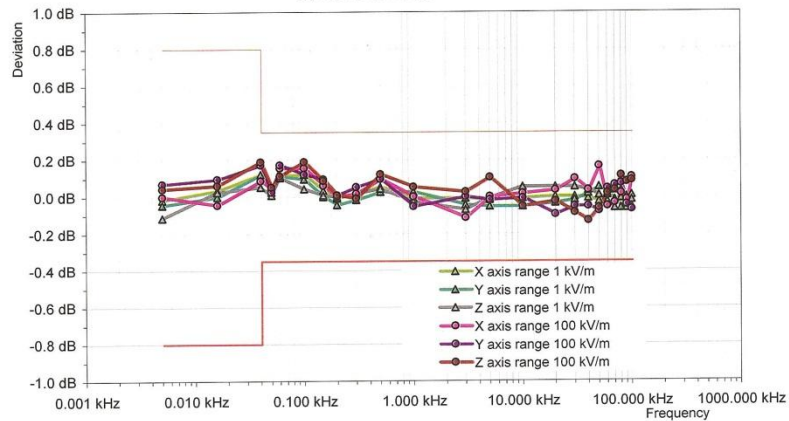
Frequency response EHP50D Electric field Measurements @ 100 V/m
