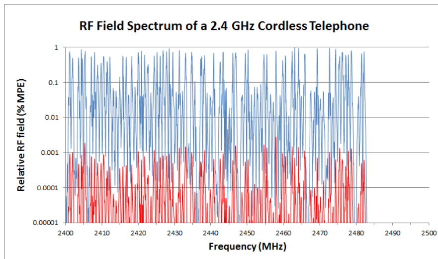
Figure 56. The relative RF field spectrum (blue is peak, red is average) of a 2.4 GHz cordless telephone at one foot from the hand set after it was turned on. RF emissions occur across a large portion of the 2.4 GHz license free band.
