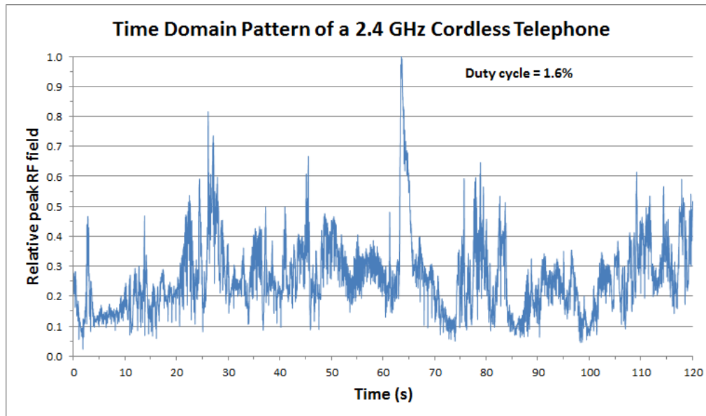
Figure 57. A measured time domain profile of the 2.4 GHz cordless telephone over a two minute (120 second) period. The duty cycle of this two minute capture of signal was 1.6%.
