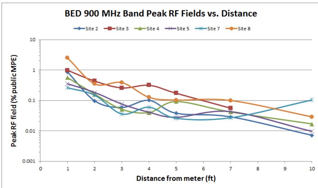
Figure 17. Logarithmic display of measured peak values of RF fields at distances up to 10 feet in front of individual smart meters operated by BED.
