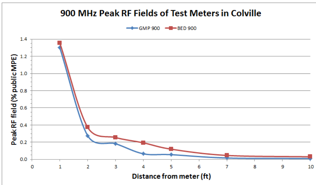
Figure 19. Measured peak RF fields produced by the Elster and Itron test meters in Colville, WA.
