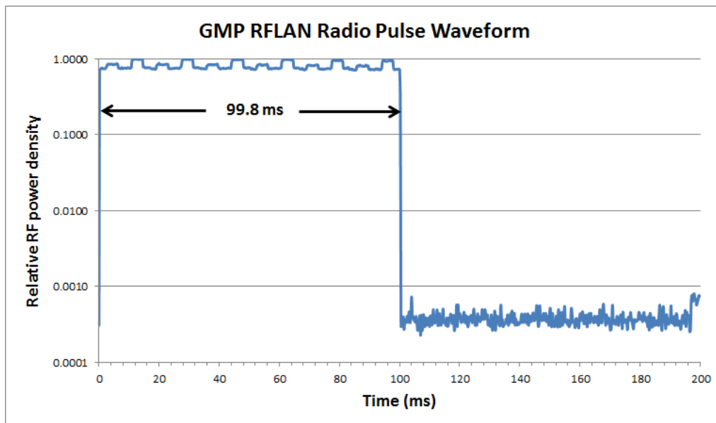
Figure 33. Waveform of GMP end point meter emission when pinged by field service unit.
