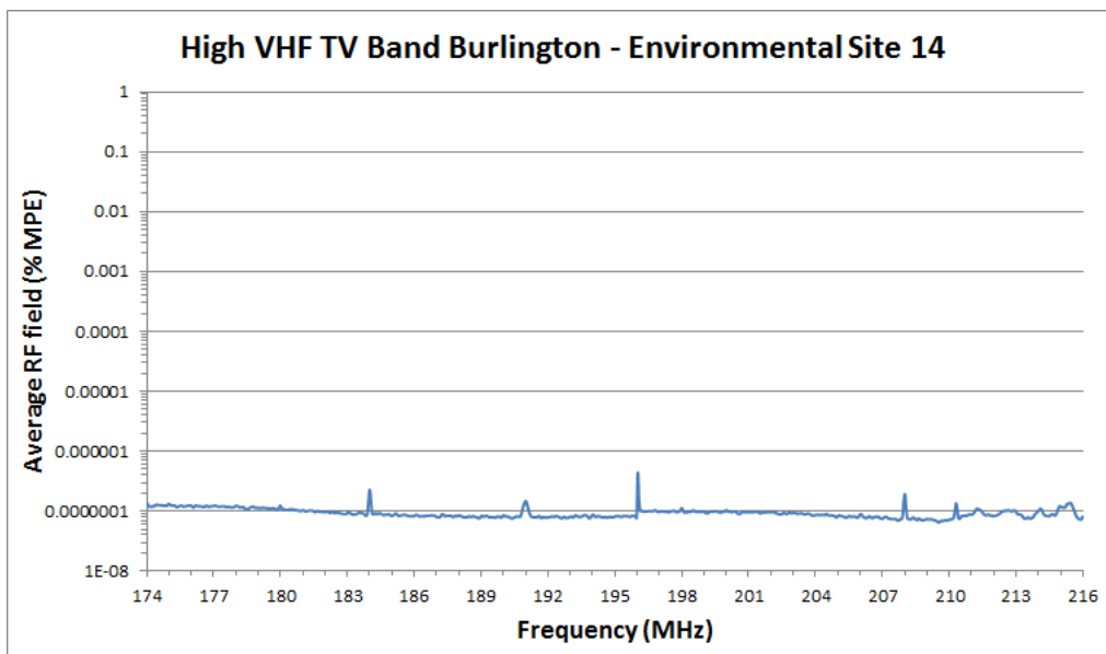
Figure 66. Spectrum measurement of average RF field (% MPE) across the high VHF TV broadcast band at environmental site 14 in Burlington.
