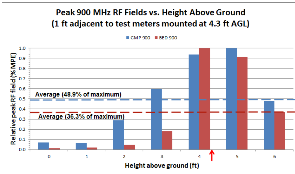
Figure 26. Relative peak 900 MHz band RF field (as a percent of the MPE) vs. height above ground at one foot in front of the Elster and Itron test meters in Colville, WA. Measured fields were normalized to the greatest value determined from all measurements.
