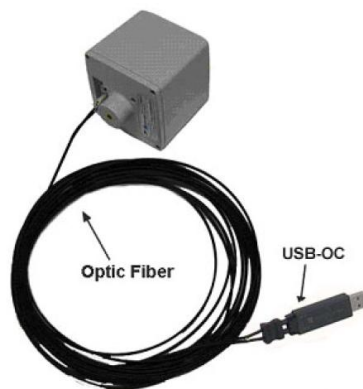
Figure 8. The Narda model EHP-50D Electric and Magnetic Isotropic Field Analyzer. The analysis of output from the sensor is performed via FFT in a connected laptop computer running special software.
