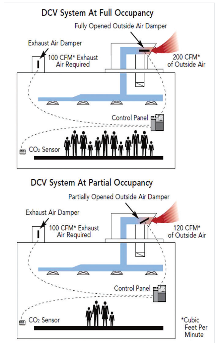
DCV system operation example
